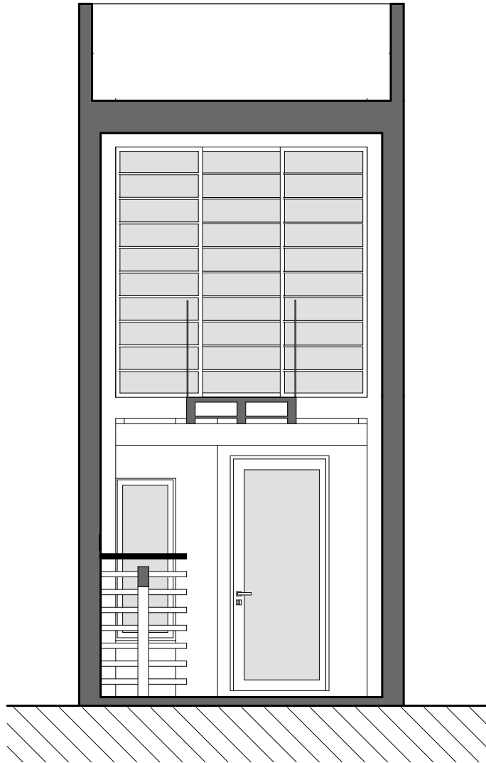
Section scale 1/50
